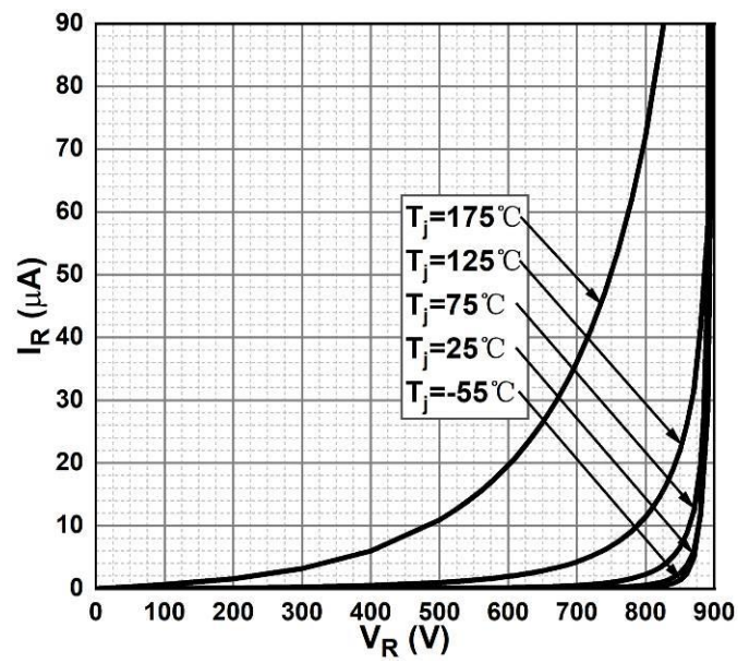
Figure 2. Reverse Characteristic
