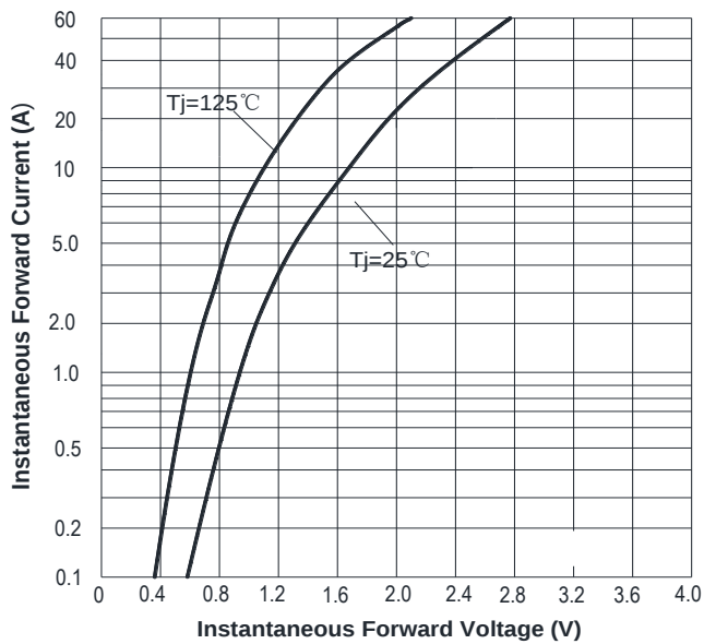
FIG3: Forward Voltage
